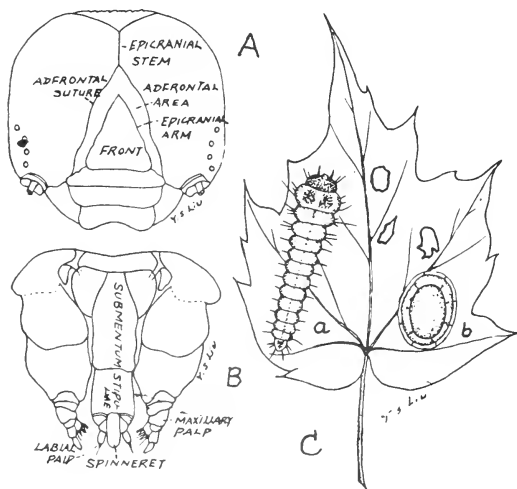
Fig. 74. A, Cephalic aspect of the head of Ceramica picta (Harr.); B, Caudal aspect of the labium of Cirphis unipuncta (Haw.); C, The maple case-bearer, Paraclemensia acerifoliella (Fitch): a, larva; b, case.
